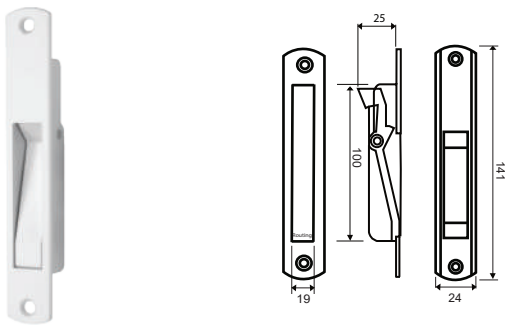
● Touch Lock L/R Code - MOZ 0915
