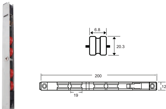
● Four Wheel Roller With Groove Code - MOZ 1754
