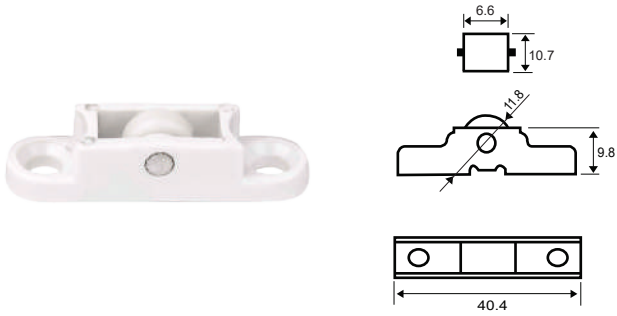
● Mesh Roller Code - MOZ 1750
