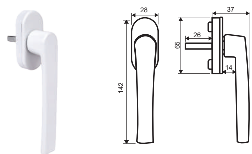
● Short Neck Handle Code - MOZ 0918
