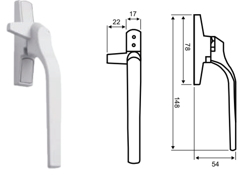
● Cockspur Handle Code - MOZ 1335
