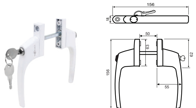
● One Side Key & One Side Knob Handle Code - MOZ 1233
