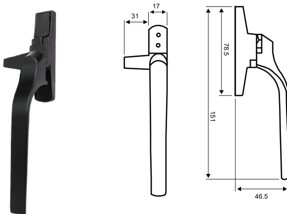
● Cockspur Handle Code - MOZ 0303
