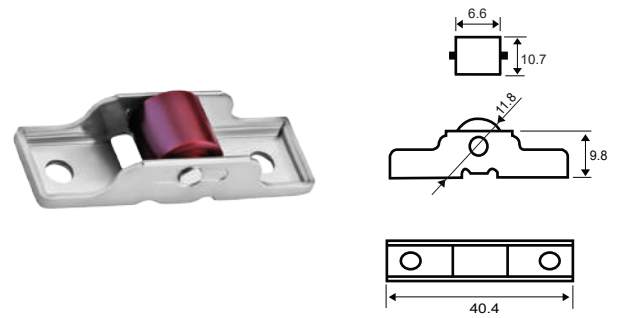
● Mesh Roller Code - MOZ 1751
