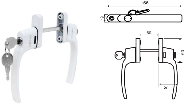
● One Side Key & One Side Knob Handle Code - MOZ 1334
