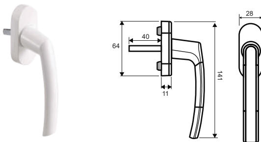
● Plastic Handle Code - MOZ 0917
