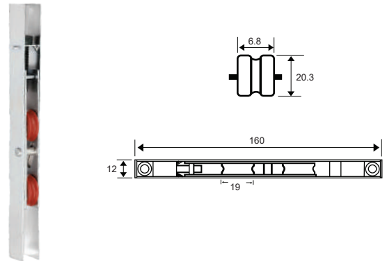
● Adjustable Nylon Double Roller Code - MOZ 1753
