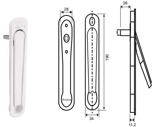
● Big Pop - up Handle Code - MOZ 1022
