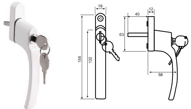
● Casement Handle With Key Code - MOZ 1231
